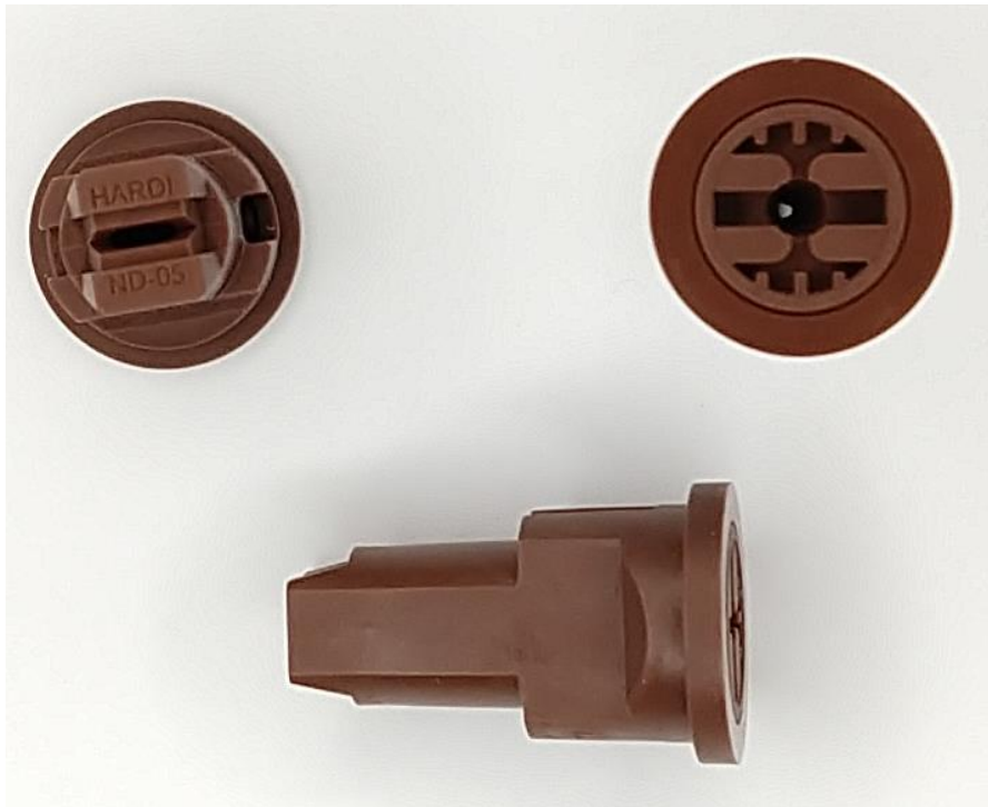
Flatfan nozzle HARDI NanoDrift ND 05 (Plastic, brown)
